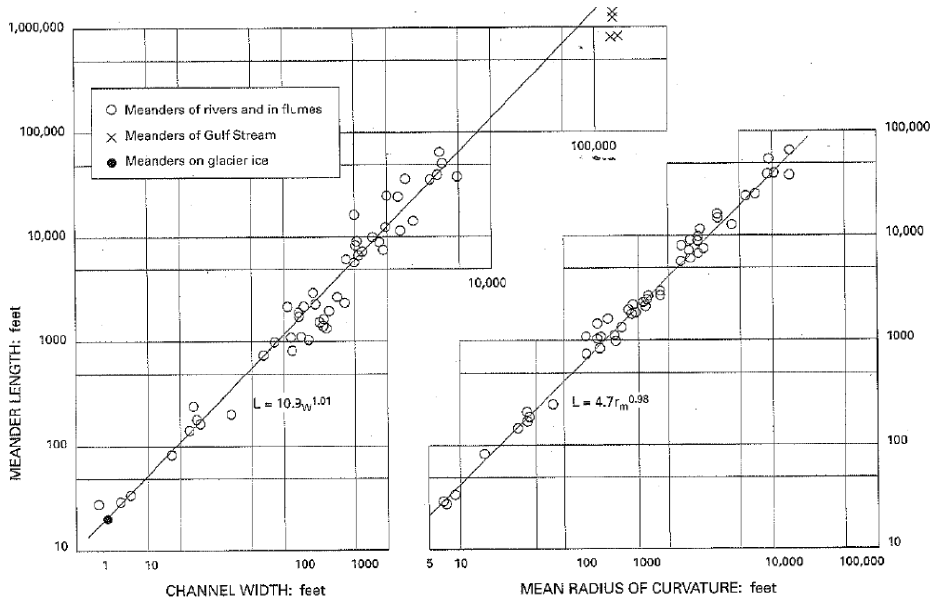
Figure 4.2 Relations between meander length and channel width, and between meander length and mean radius of curvature.
