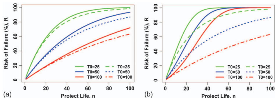
Fig. 8. (Color) Nonstationary risk of failure as a function of project life n (assuming initial designs for T_0 = 25, 50, and 100 years; the dashed lines show the risk for the stationary condition, whereas the solid lines show the risk for nonstationary conditions): (a) Aberjona River Basin (assuming the GEV model); (b) Little Sugar Creek Basin (assuming the Gumbel model)
