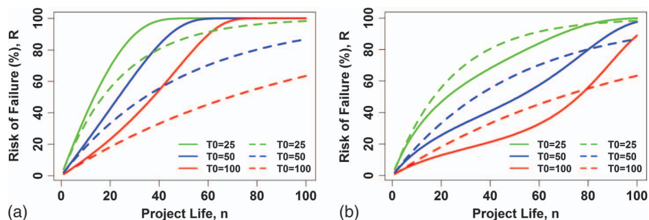
Fig. 11. (Color) Increase in risk of failure R as a function of project life n (the dashed lines show the risk for the stationary condition, whereas the solid lines show the risk for nonstationary conditions): (a) Key West; (b) Adak
